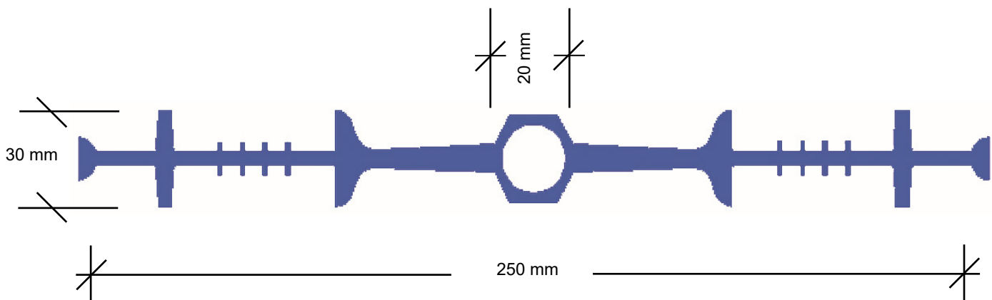
Center fix for expansion & construction joints (AB234)
