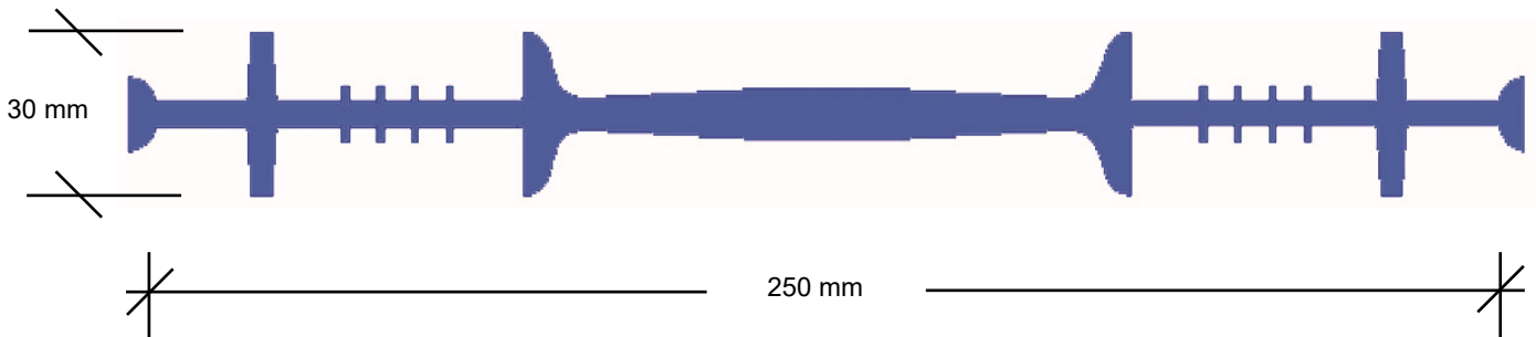
Center fix for construction joints (AB233)
